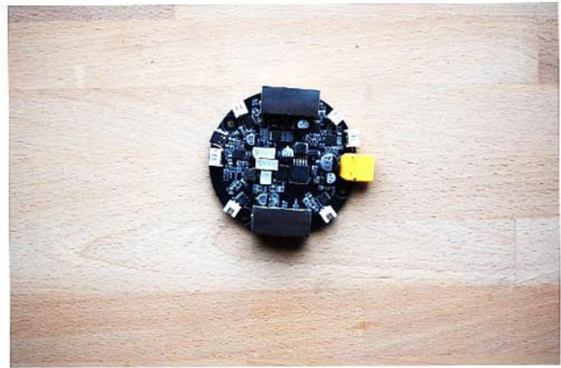
Five Axis Control Board. Quantity 1. Properties: Four servo axis, one stepper axis (dual drive), four ethernet encoder
