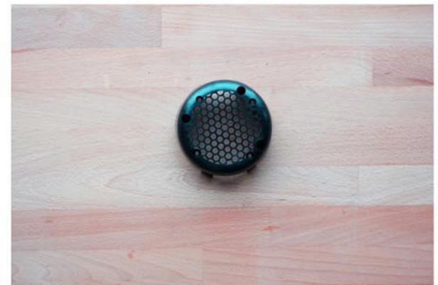
PCB Enclosure Top. Quantity 1. Properties: Glass fiber reinforced polycarbonate.
